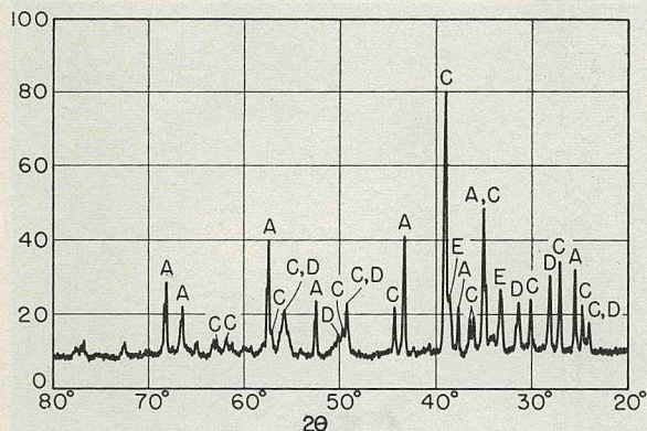
Fig. 12. X-ray diffraction pattern of 100% \text{ZrSiO}_4 thermite pellet after ignition. A = \text{Al}_2\text{O}_3 , C = \text{ZrSi}_2 , D = \text{ZrO}_2 , and E = \text{ZrN} or \text{ZrO} . Peaks designated \text{ZrN} or \text{ZrO} correspond to a NaCl-type lattice with cell edge of about 4.64 a.u. Pattern was obtained with a North American Philips diffractometer using copper radiation filtered through nickel foil.
