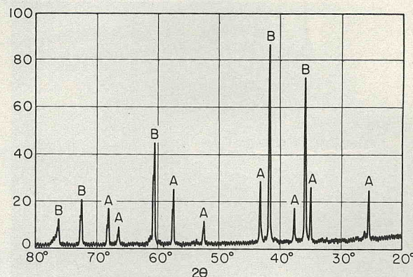
Fig. 13. X-ray diffraction pattern of 100% \text{TiO}_2 carbon thermite pellet after ignition. A = \text{Al}_2\text{O}_3 and B = \text{TiC} . Pattern was obtained as indicated in Fig. 12.
